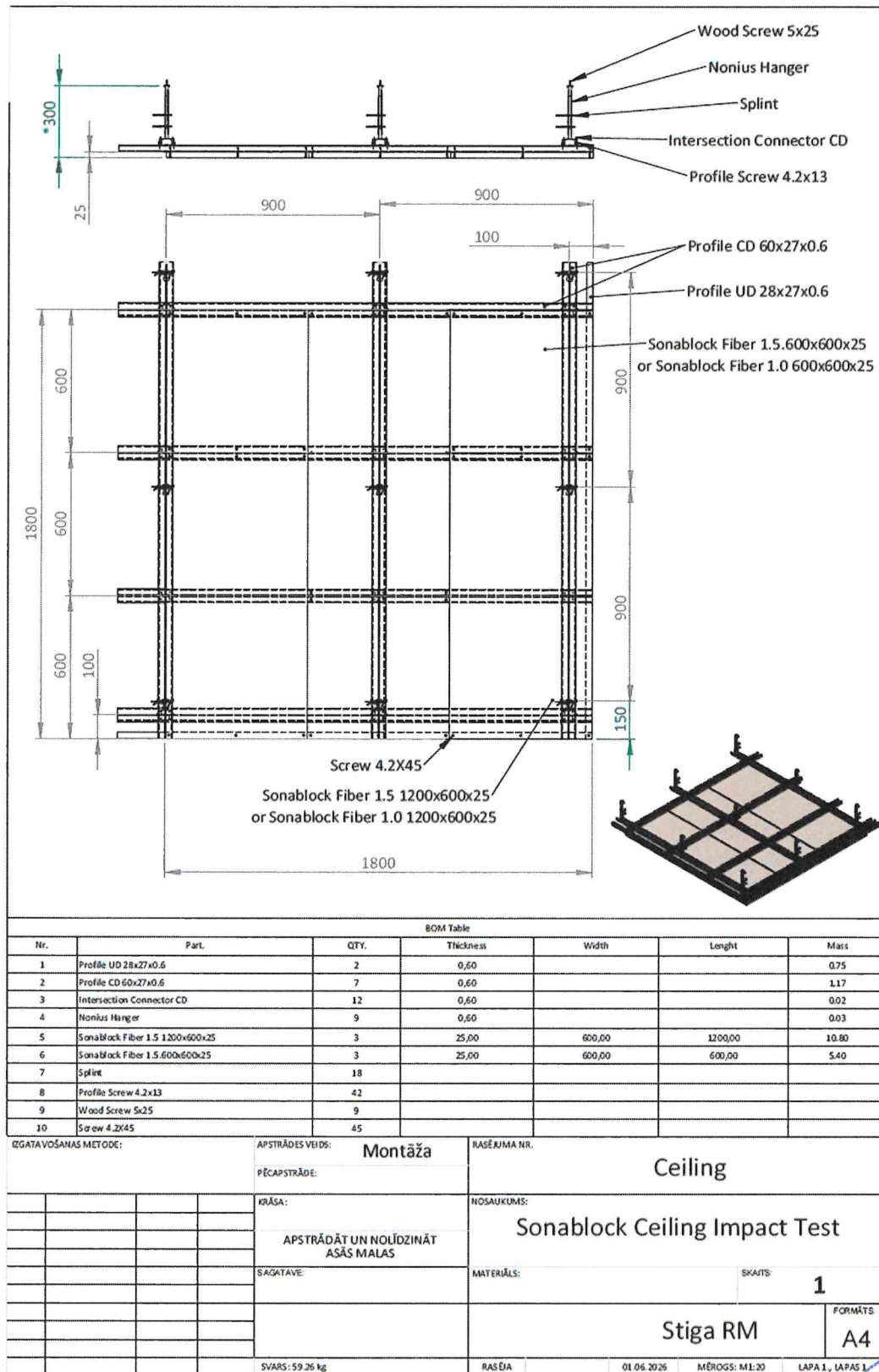
drawing 1 of the tested ceiling paneling "Sonablock Fiber 1.0"
